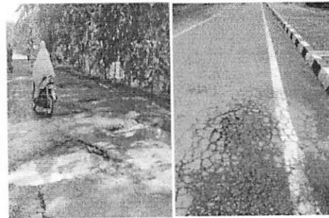
Fig. 1: Expansive soil conditions on the Takalar-Jenepono highway
